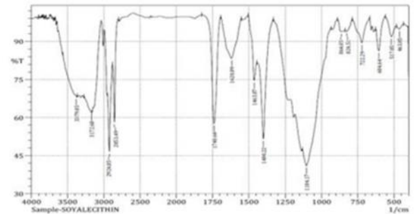
Figure 4: FT – IR of lecithin
