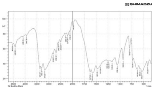
Figure 2: FT – IR of pure Metformin
