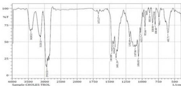
Figure 3: FT – IR of cholesterol
