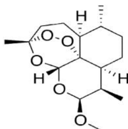
Fig. 2: Molecular structure of Artemether
