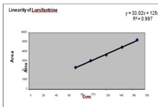
Fig. 5: Linearity graph of Lumefantrine
