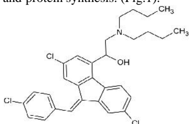
Fig. 1: Molecular structure of Lumefantrine
