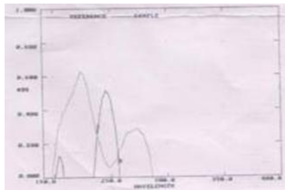
Fig. 3: Overlain UV Spectra for Lumefantrine and Artemether
