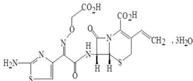
Figure 1: Structural formula of Cefixime Trihydrate
