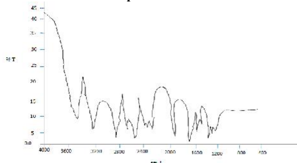
Figure 4: IR Absorbance spectra of diacid ( 2a ) i.e. [2a, (2Z, 3Z)-2-3-bis(4-chlorophenyl)( phenyl) (methylene) succinic acid)]
