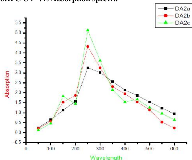
Figure 7: UV-Vis Absorption spectra of diacids (2a, 2b, 2c)
