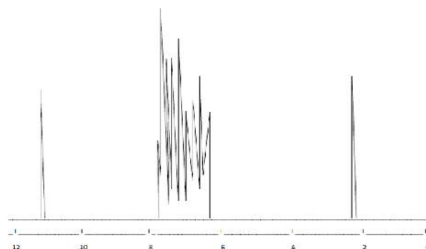
Figure 1: Proton NMR Spectra of diacid ( 2a ) i.e. [2a, (2Z, 3Z)-2-3-bis(4-chlorophenyl)( phenyl) (methylene) succinic acid)]
