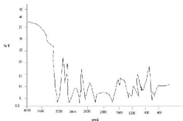
Figure 6: IR Absorption spectra of diacid (2c) i.e. [2c, (2Z, 3E)-2-3-bis (furan-2-ylmethylene) succinic acid]
