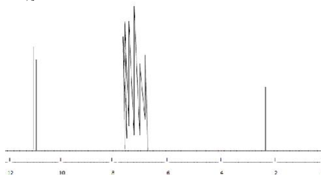
Figure 2: Proton NMR Spectra of diacid ( 2b ) i.e. [2b, (2Z, 3Z)-2-(4-chlorophenyl)(phenyl)(methylene)-3-(1-phenyl ethylidene) succinic acid]
