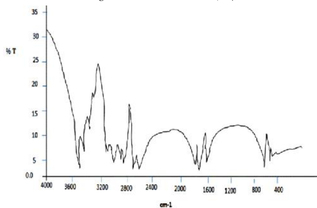
Figure 5: IR Absorption spectra of diacid (2b) i.e. [2b, (2Z, 3Z)-2-(4-chlorophenyl) (phenyl) (methylene)-3-(1-phenyl ethylidene) succinic acid]
