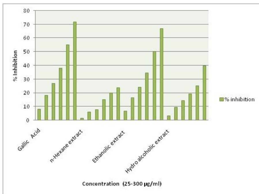
Figure 2: Hydrogen peroxide scavenging activity of Merremia turpethum
