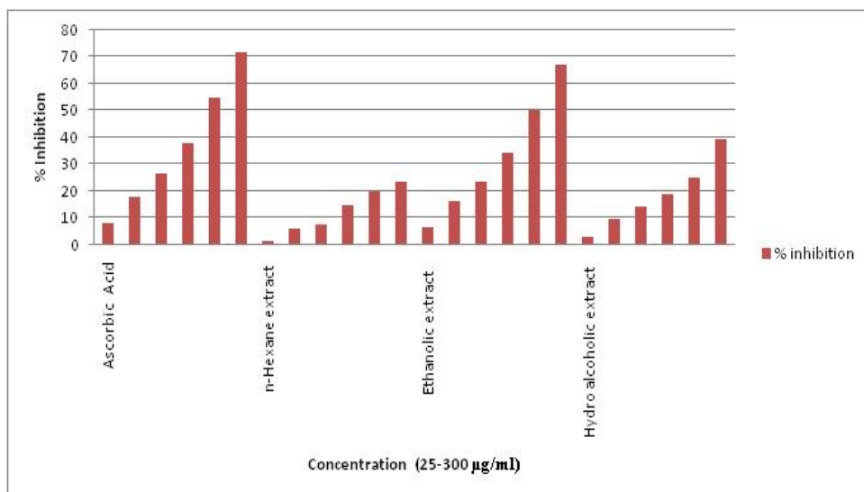
Figure 1: DPPH radical scavenging activity of Merremia turpethum
