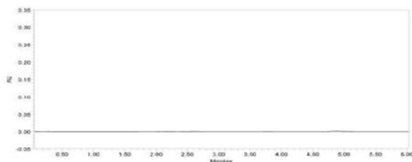
Chromatogram of Blank
