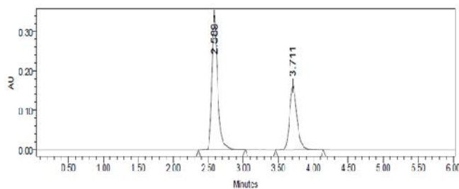
Chromatogram of Sample
