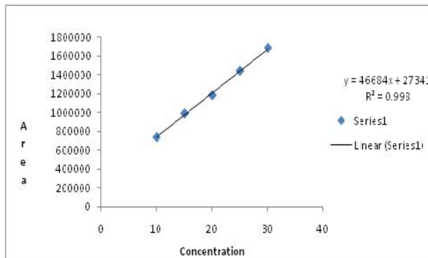
Calibration graph of Perindopril
