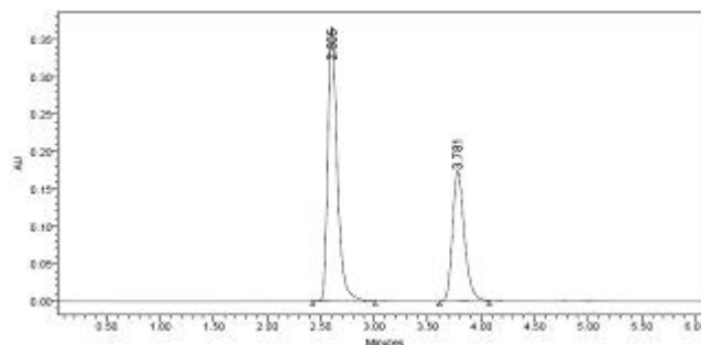
Figure 3: Optimization Chromatogram
