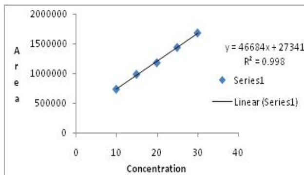
Calibration graph of Amlodipine
